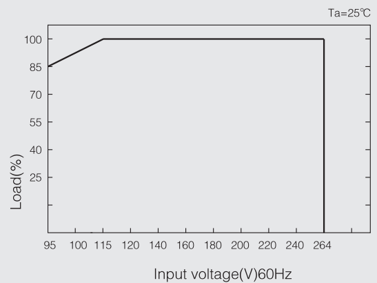
Static characteristic
